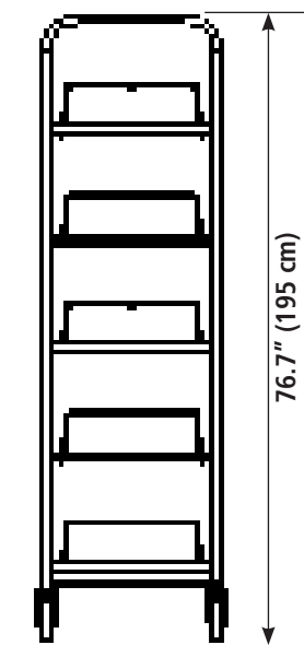
Front Elevation Model USR60
